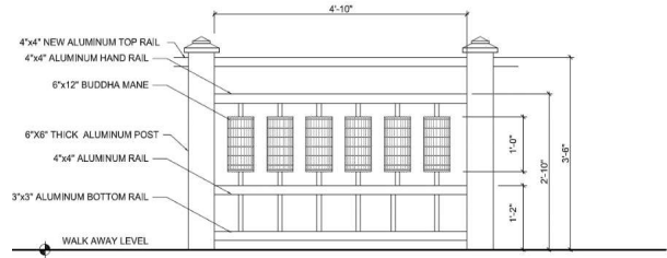
6 NOS - MANE RAILING ELEVATION OPTION - 1
