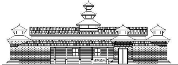
SIDE ENTRANCE - SIDE ELEVATION
